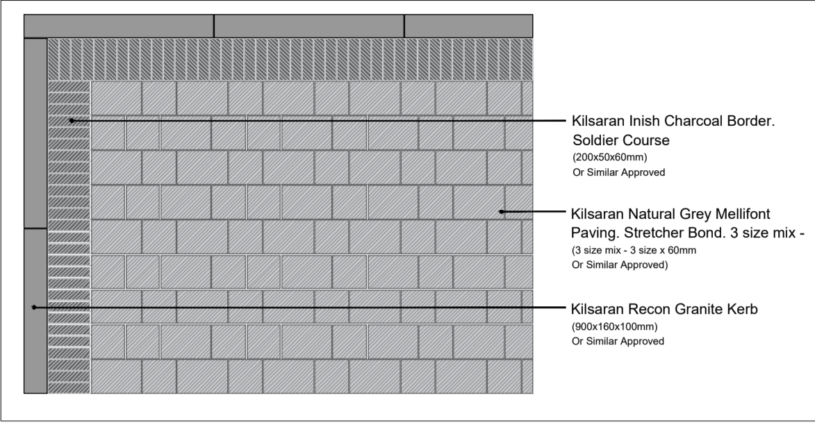
Paving Detail 1 Scale : 1:25 @ A1
