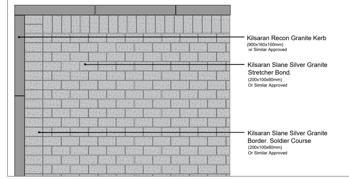
Paving Detail 8 Scale : 1:25 @ A1
