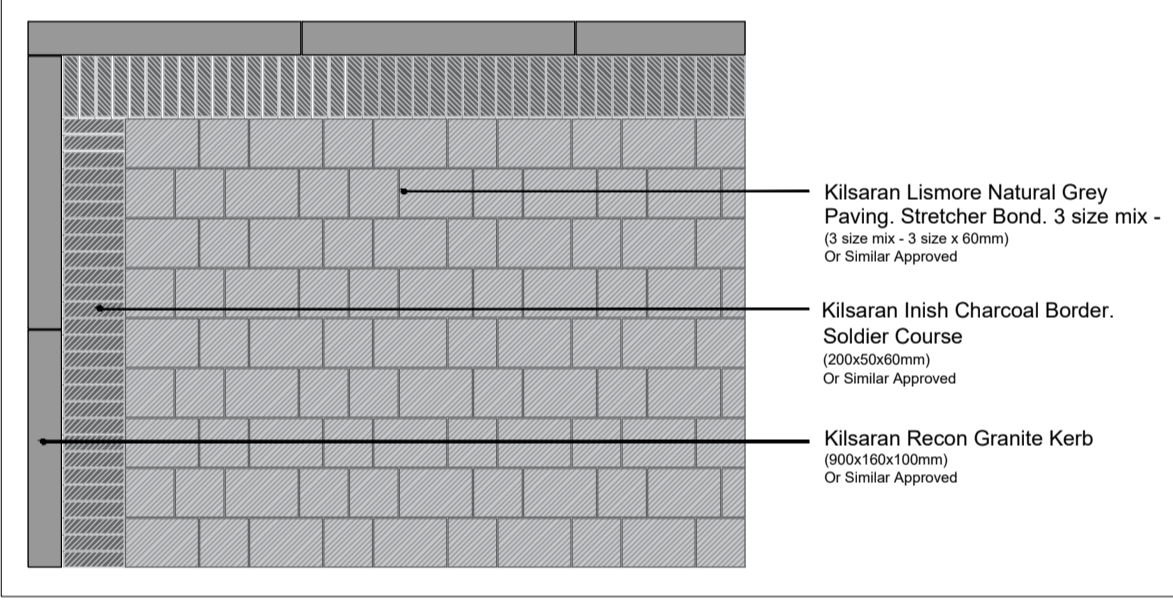
Paving Detail 3 Scale : 1:25 @ A1
