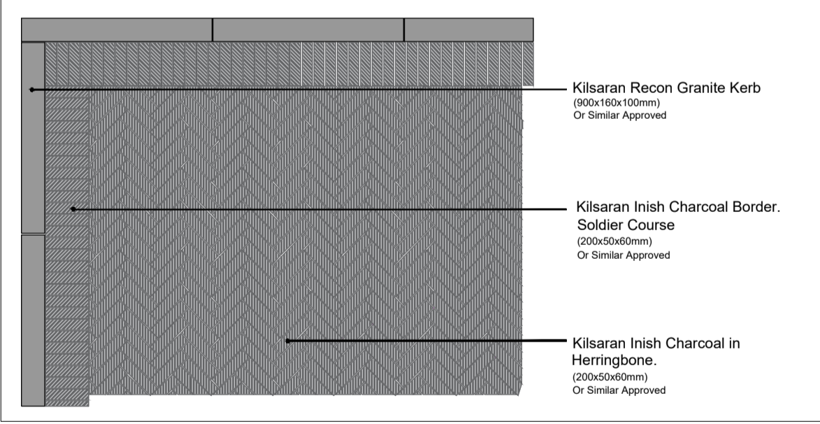
Paving Detail 4 Scale : 1:25 @ A1
