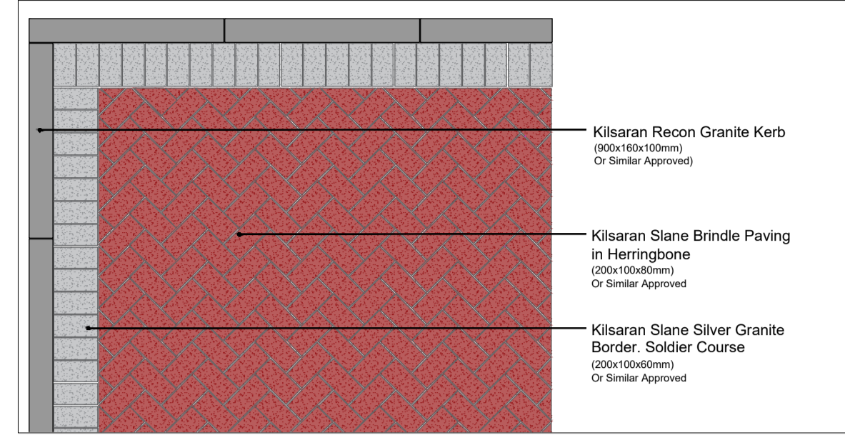
Paving Detail 6 & 7 Scale : 1:25 @ A1
