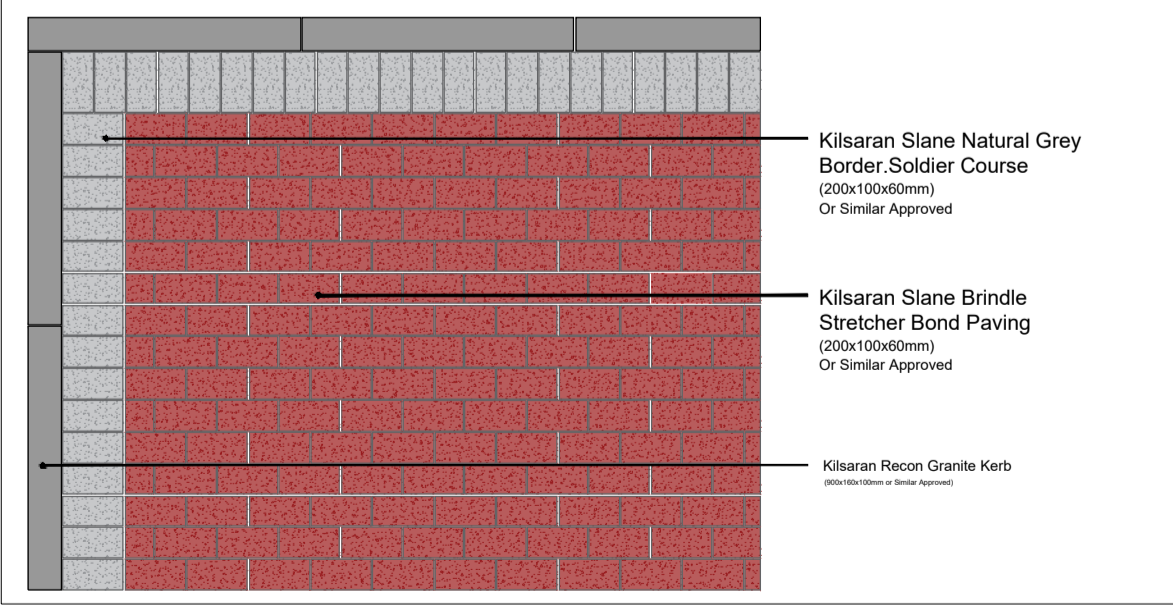
Paving Detail 5 Scale : 1:25 @ A1
