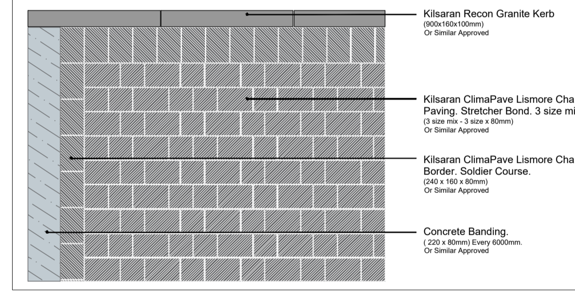
Paving Detail 9 Scale : 1:25 @ A1
