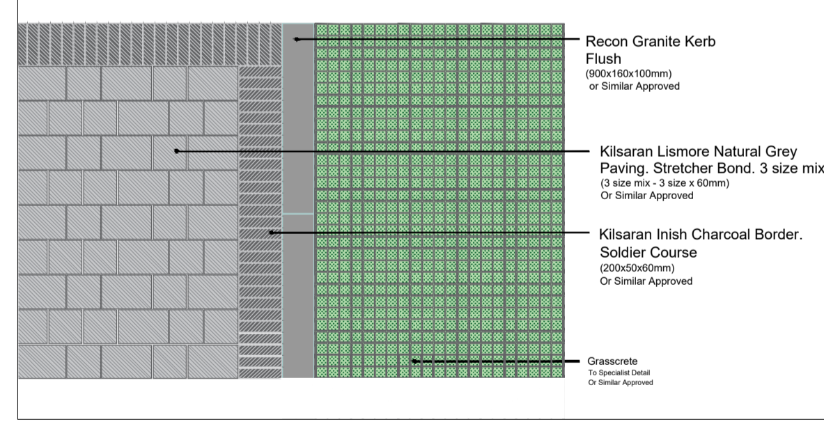
Paving Detail 10 Scale : 1:25 @ A1
